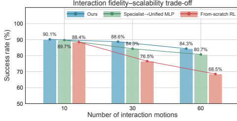
Figure 5: Fidelity–scalability trade-off.
