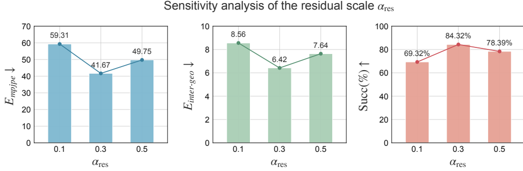
Figure 9: Sensitivity to the residual action scale \alpha_{\text{res}} . A scale of 0.3 achieves the lowest tracking and interaction geometry errors and the highest success rate.
